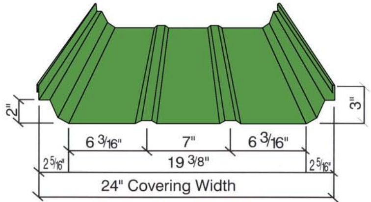
Guardian Profile
