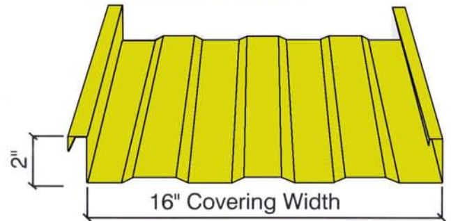
Sure-Lok Profile
