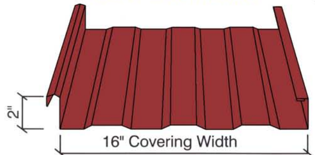
Supreme-Lok Profile
