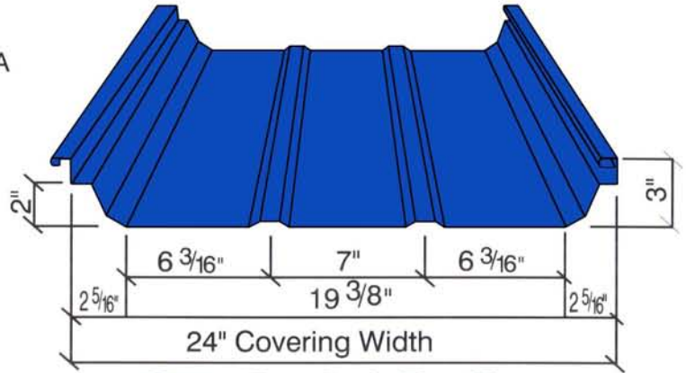
Guardian-Lok Profile
